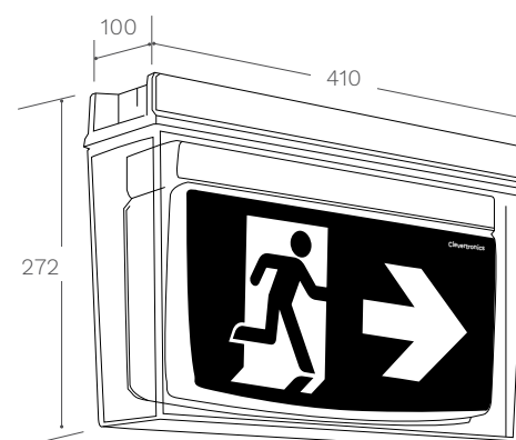
Dimensions (mm)
